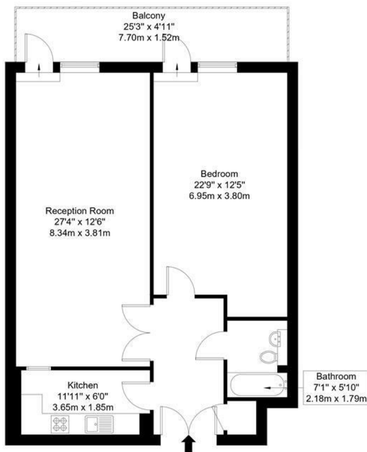
Second Floor
