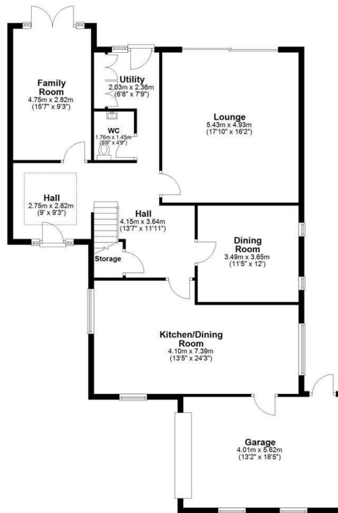
Ground Floor Approx. 138.4 sq. metres (1468.7 sq. feet)
