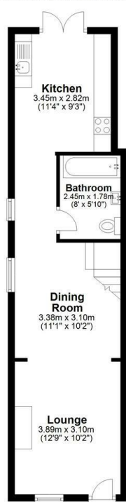
Ground Floor Approx. 40.7 sq. metres (438.6 sq. feet)
