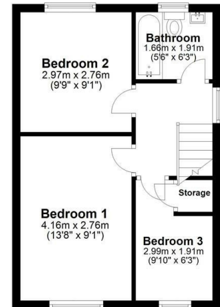
First Floor Approx. 34.5 sq. metres (371.5 sq. feet)
