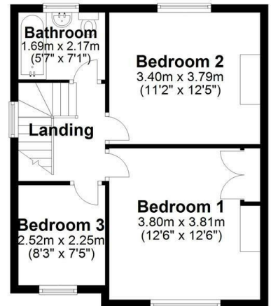
First Floor Approx. 43.5 sq. metres (468.4 sq. feet)
