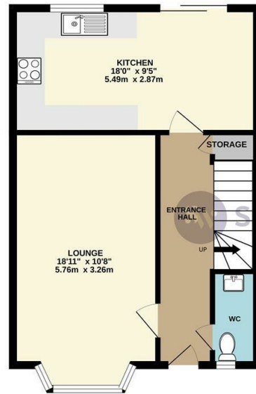
GROUND FLOOR 485 sq.ft. (45.1 sq.m.) approx.
