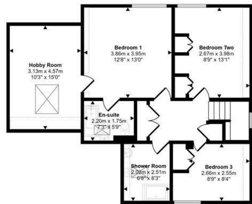
First Floor Approx 72 sq m / 779 sq ft
