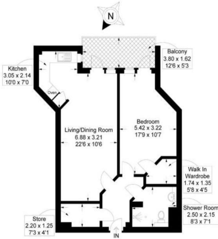
Second Floor
