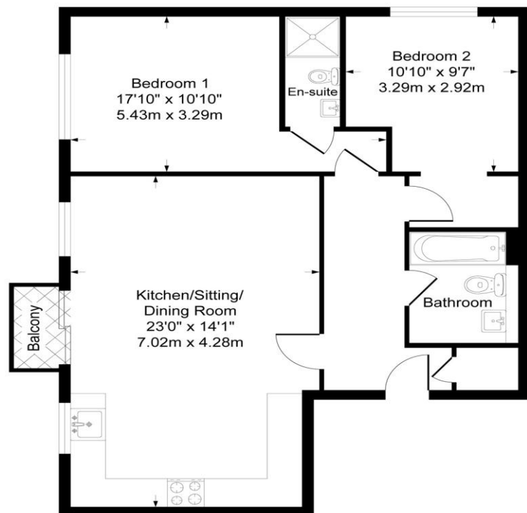
Second Floor
