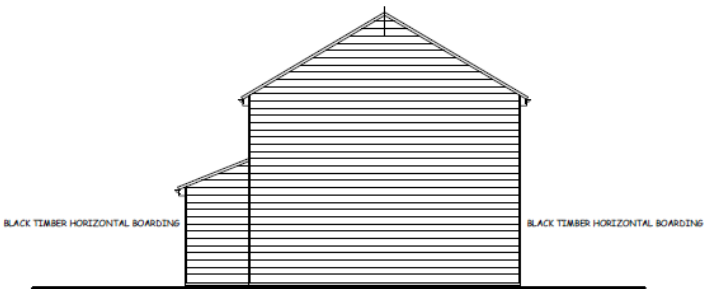
SIDE ELEVATION 1/100 scale.
