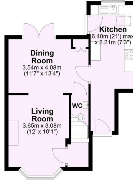
Ground Floor Approx. 44.2 sq. metres (475.9 sq. feet)
