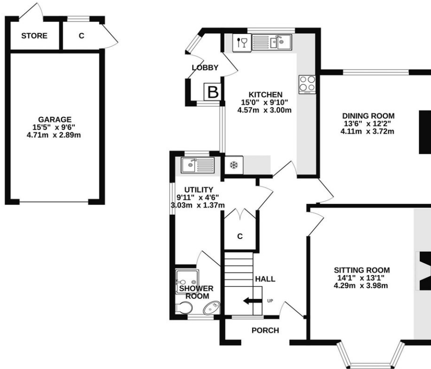
GROUND FLOOR 942 sq.ft. (87.5 sq.m.) approx.
