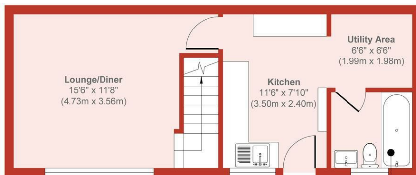
Ground Floor Approximate Floor Area 352 sq. ft (32.75 sq. m)
