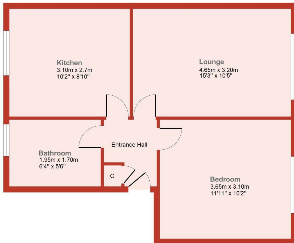
Floor Plan
