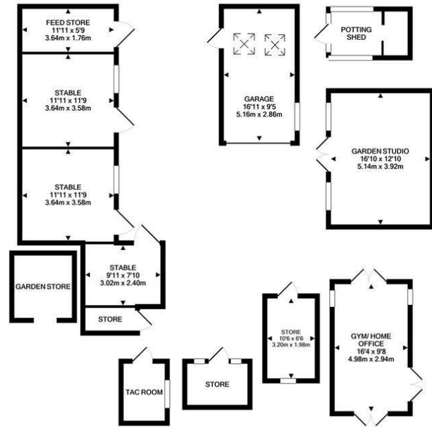
OUTBUILDINGS APPROX. FLOOR AREA 1265 SQ.FT. (117.6 SQ.M.)
