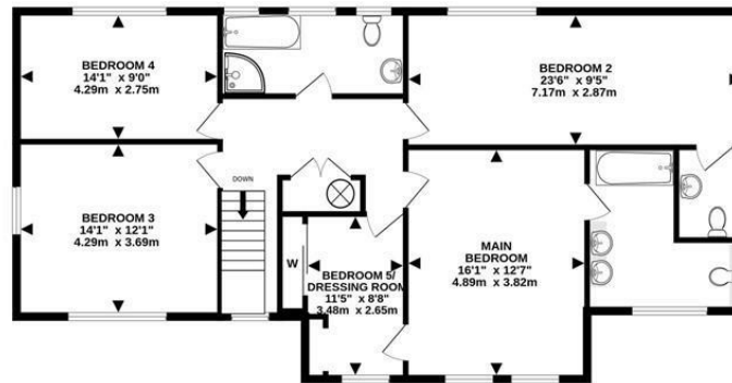
1ST FLOOR
