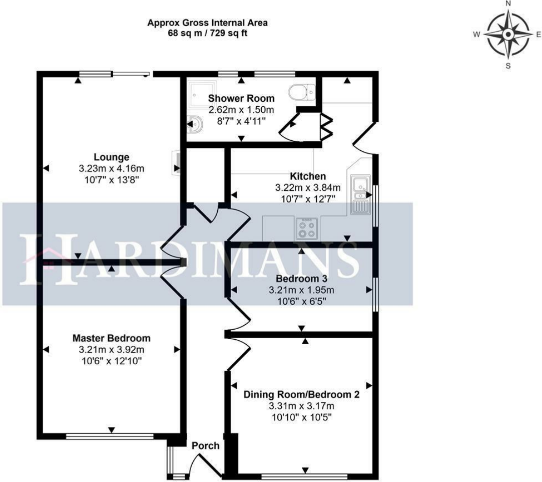
Floorplan
