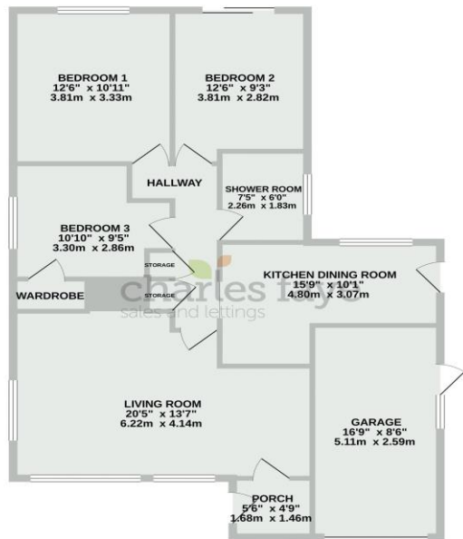
TOTAL FLOOR AREA: 1001 sq.ft. (93.0 sq.m.) approx. Made with Mapbox ©2025
