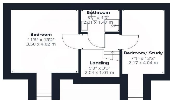
Floor 2 Building 1
