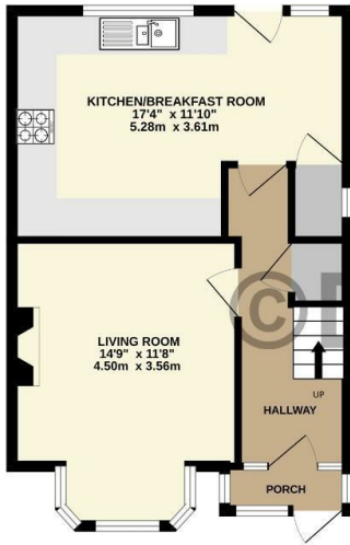
GROUND FLOOR 437 sq.ft. (40.6 sq.m.) approx.
