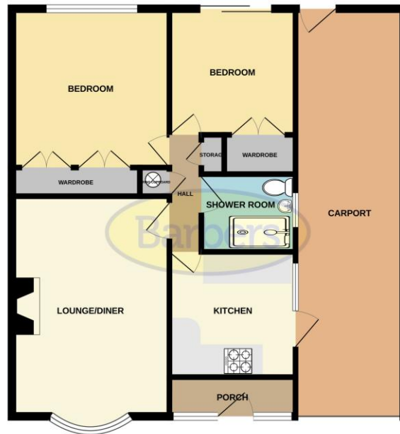
GROUND FLOOR 773 sq.ft. (71.8 sq.m.) approx.
