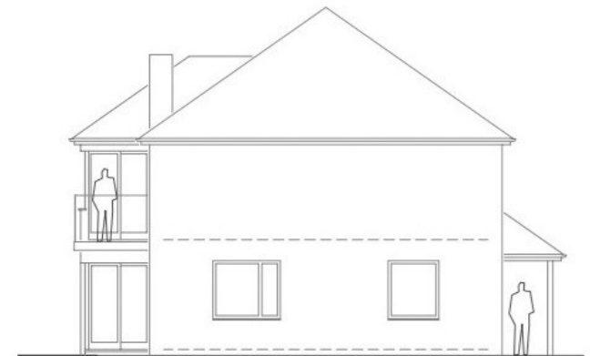
SOUTH–WEST ELEVATION
