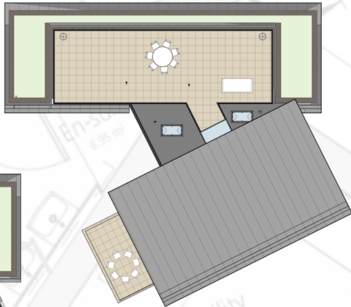
TRESCO ROOF PLAN
