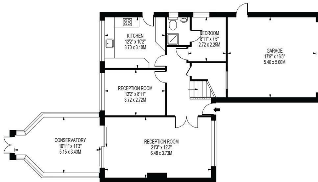
GROUND FLOOR
