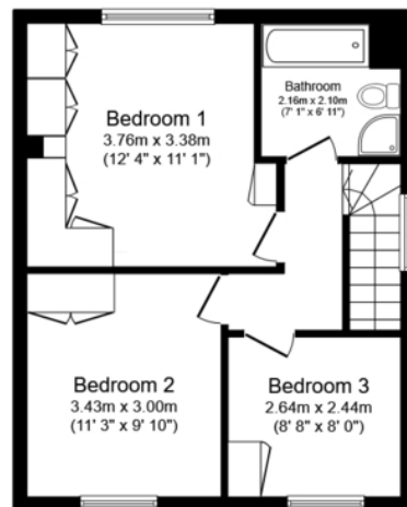
First Floor Floor area 42.2 sq.m. (454 sq.ft.)
