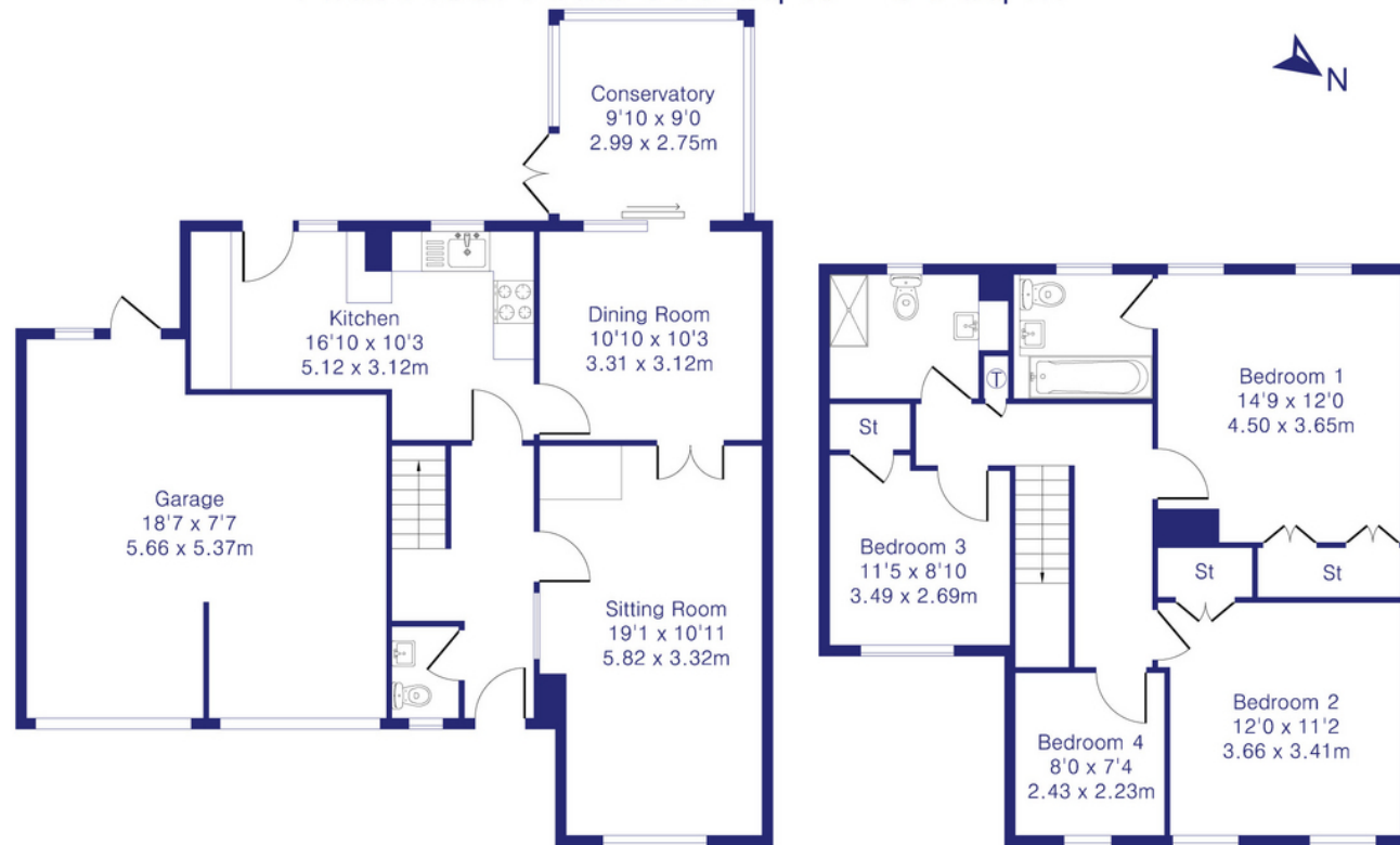
Ground Floor
