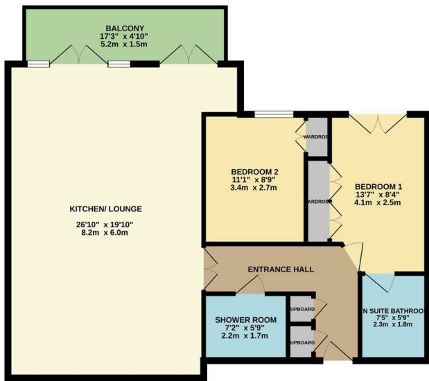
GROUND FLOOR 863 sq.ft. (80.2 sq.m.) approx.
