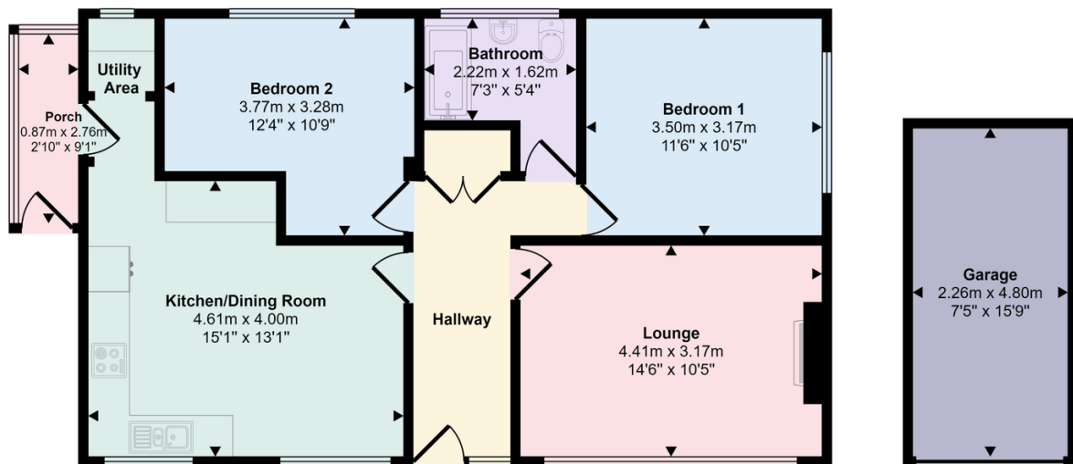
Floorplan
