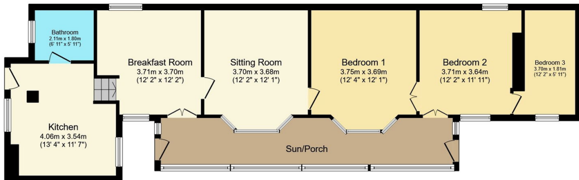
Floor Plan
