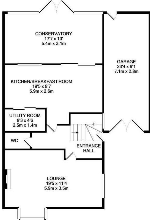
GROUND FLOOR APPROX. FLOOR AREA 958 SQ.FT. (89.0 SQ.M.)
