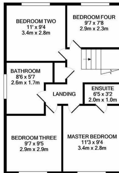
1ST FLOOR APPROX. FLOOR AREA 539 SQ.FT. (50.1 SQ.M.)
