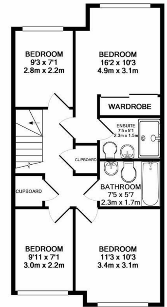
1ST FLOOR APPROX. FLOOR AREA 569 SQ.FT. (52.8 SQ.M.)
