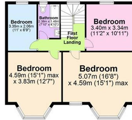
First Floor Approx. 67.0 sq. metres (721.5 sq. feet)
