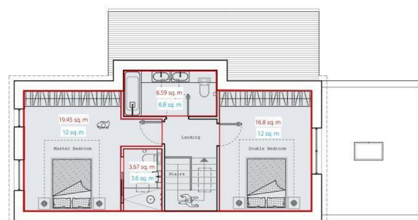
First Floor Plan Gross internal floor area of 51.39 sqm
