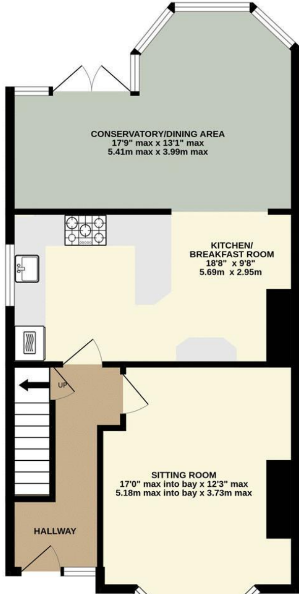
GROUND FLOOR 611 sq.ft. (56.8 sq.m.) approx.
