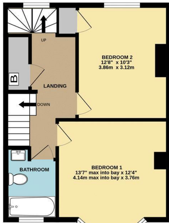
1ST FLOOR 437 sq.ft. (40.6 sq.m.) approx.
