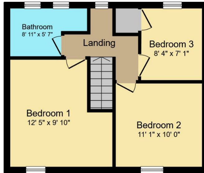
First Floor Floor area 406 sq.ft.
