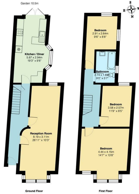
Total Area: 96.7 m 2 ... 1041 ft 2 All measurements are approximate and for display purposes only.
