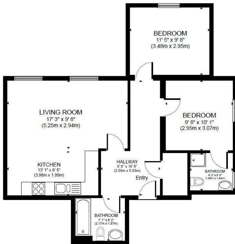
FLOOR PLAN
