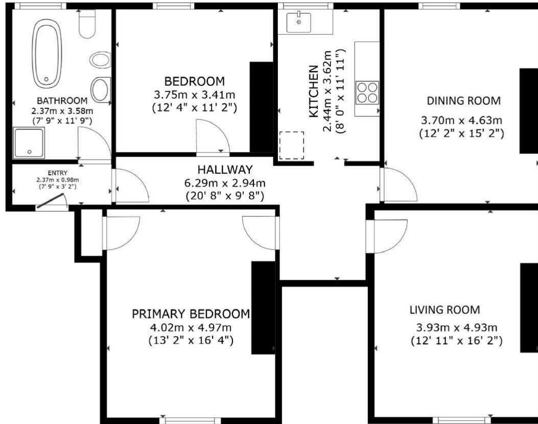
FLOOR PLAN
