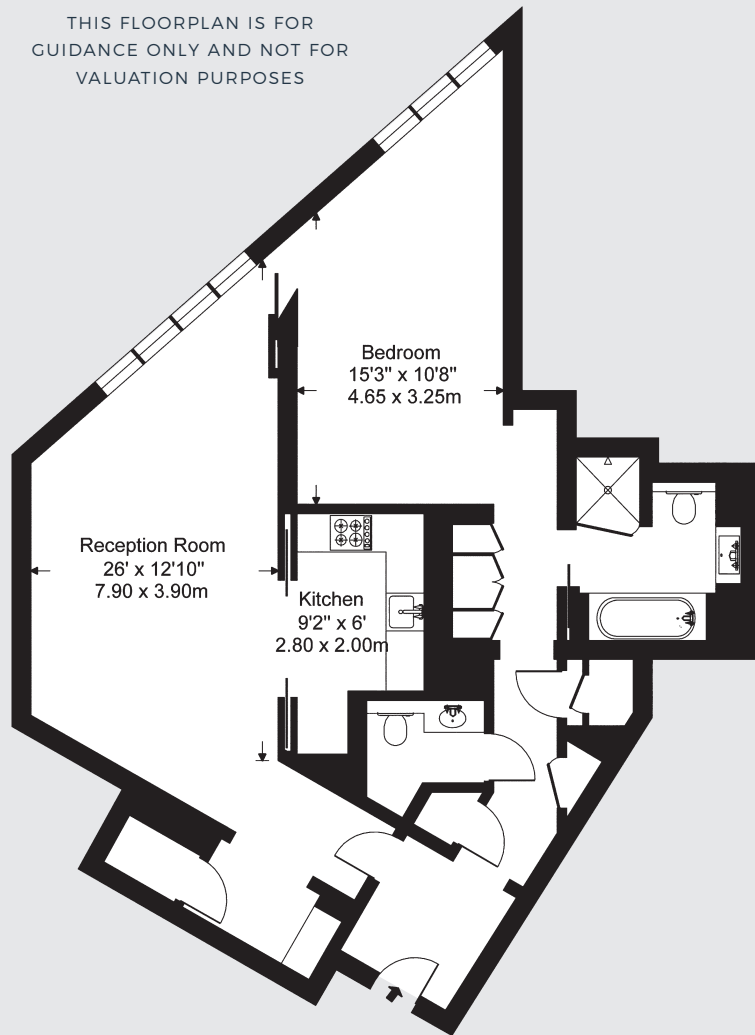
FOURTH FLOOR
