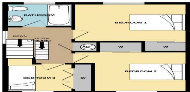
1ST FLOOR 445 sq.ft. (41.3 sq.m.) approx.
