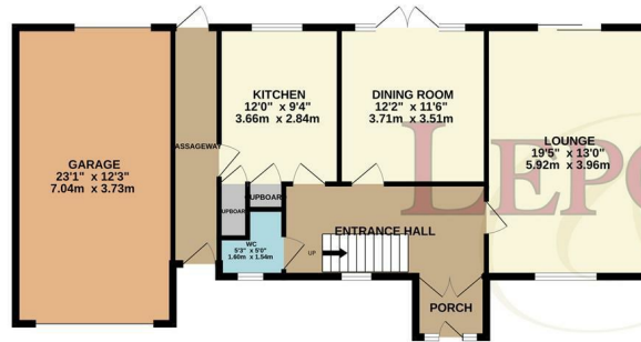
GROUND FLOOR 1030 sq.ft. (95.7 sq.m.) approx.
