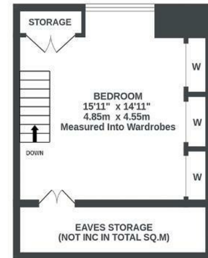
2ND FLOOR 229 sq.ft. (21.3 sq.m.) approx.
