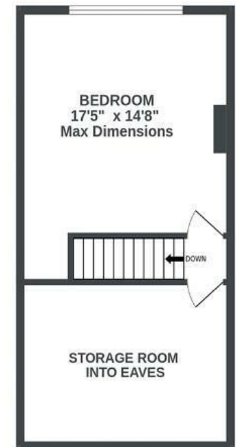
2ND FLOOR 406 sq. ft. approx.
