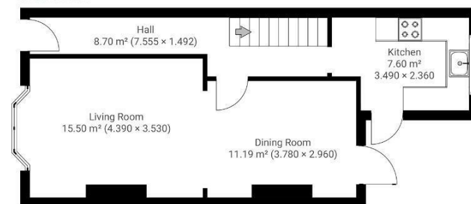
GROUND FLOOR
