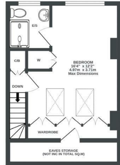
2ND FLOOR 263 sq.ft. (24.5 sq.m.) approx.
