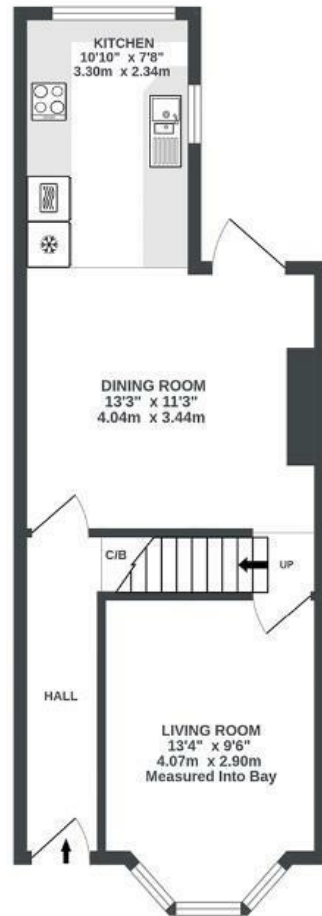
GROUND FLOOR 421 sq ft (38.1 sq m) approx.
