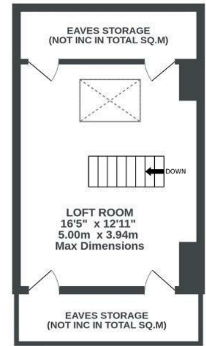
2ND FLOOR 205 sq.ft. (19.0 sq.m.) approx.
