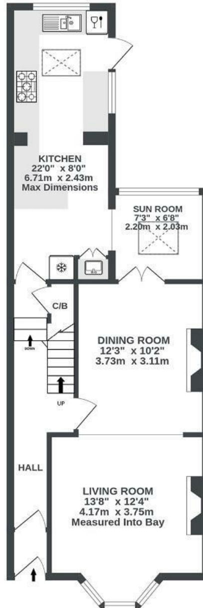
GROUND FLOOR 587 sq.ft. (54.5 sq.m.) approx.
