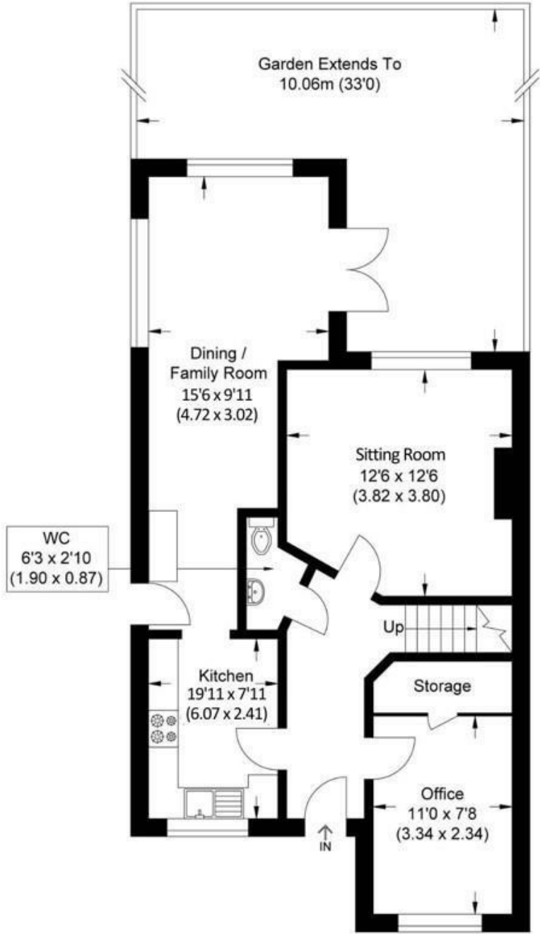
Ground Floor
