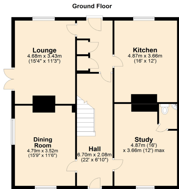
Floorplan of existing building. Plan produced using PlanUp.
